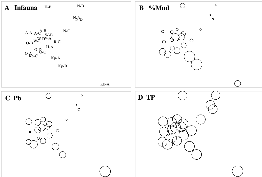
Figure A31: MDS ordination of the Bray-curtis similarities of infauna data (A), and the same ordination superimposed with circles of increasing size with increasing content of the environmental parameters, %Mud (B), Lead, Pb (C) and total phosphorus, TP (D). Data were presented as un-normalised, raw data.
