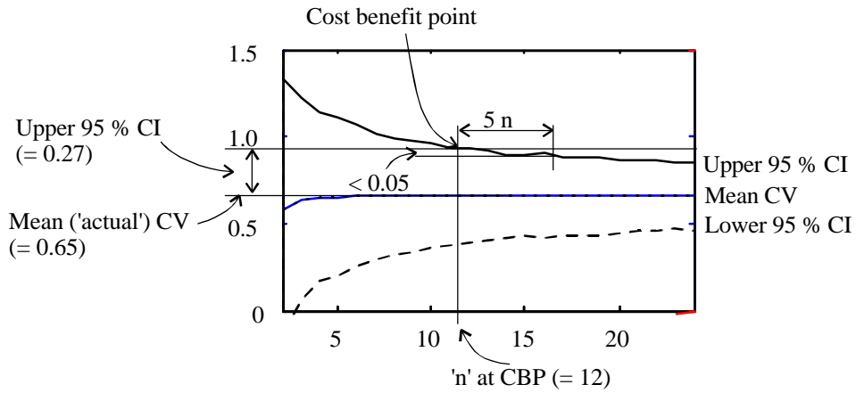
Figure A30: An example of how the cost benefit point (CBP) and near 'actual CV' are derived from a randomized plot of mean CV \pm 95 % CI with increasing sample number.
