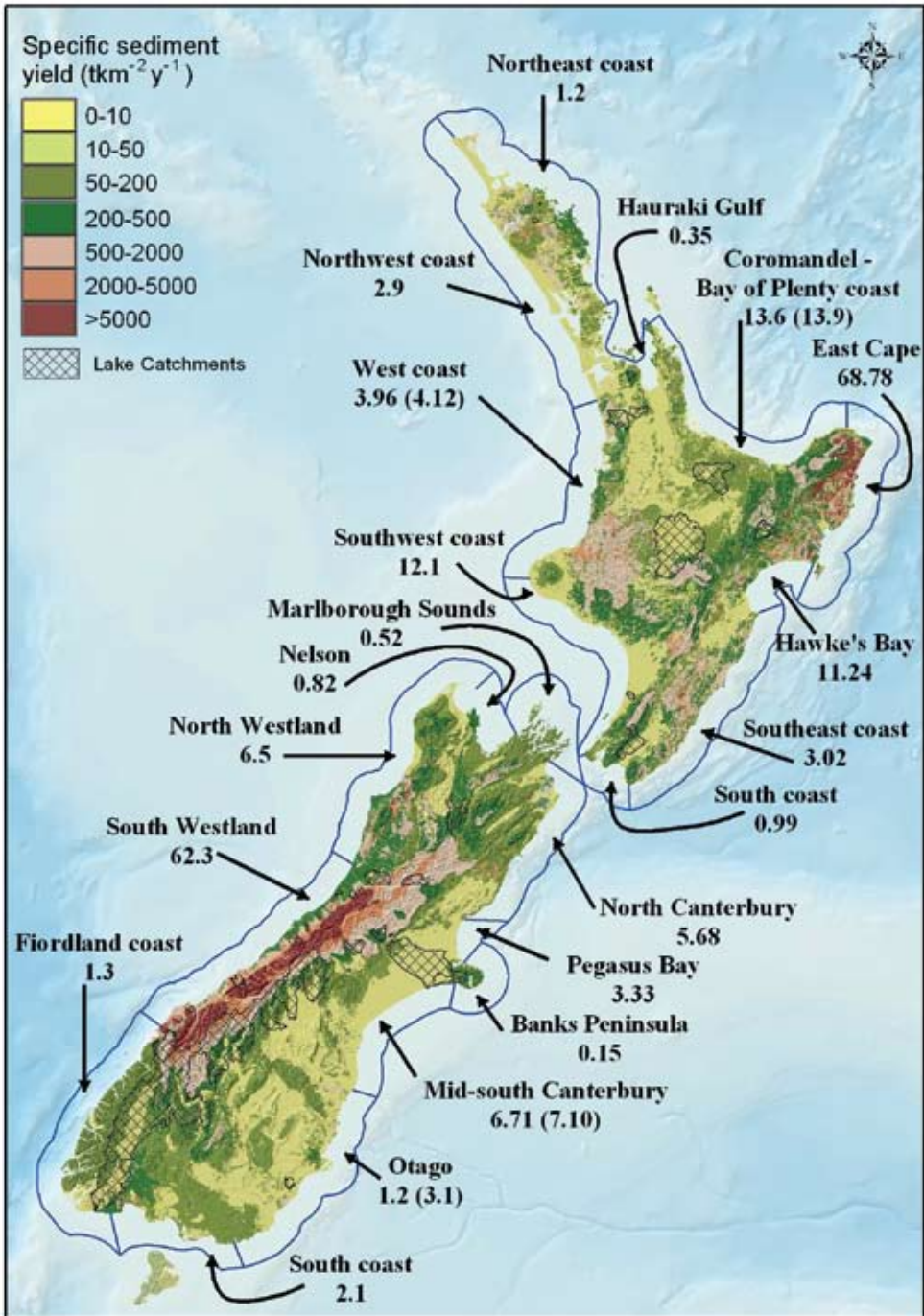
Figure 10 – Raster map of specific yield of river suspended sediment generated by empirical GIS model and sediment yields to coast (Mt/y) totalled by region. Yield totals are adjusted for sediment entrapment in natural lakes and hydro-lakes. Figures in brackets give yields without hydro-lakes. Hatched areas show large natural lake catchments.
