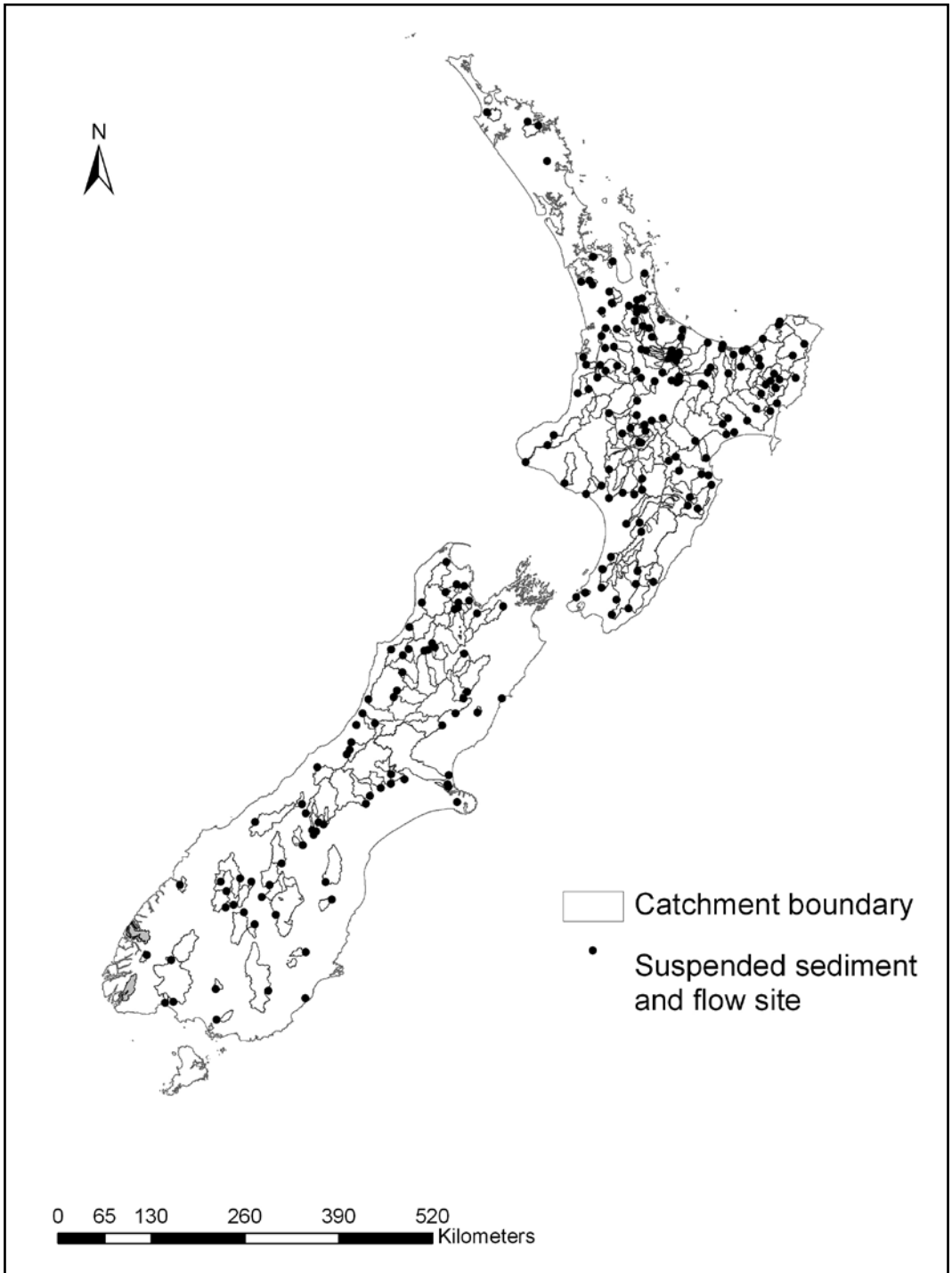
Figure 1 – River suspended sediment gauging and flow recording sites and catchments, and catchments contributing to fiord and lake sediment traps. Fiord catchments are shaded.
