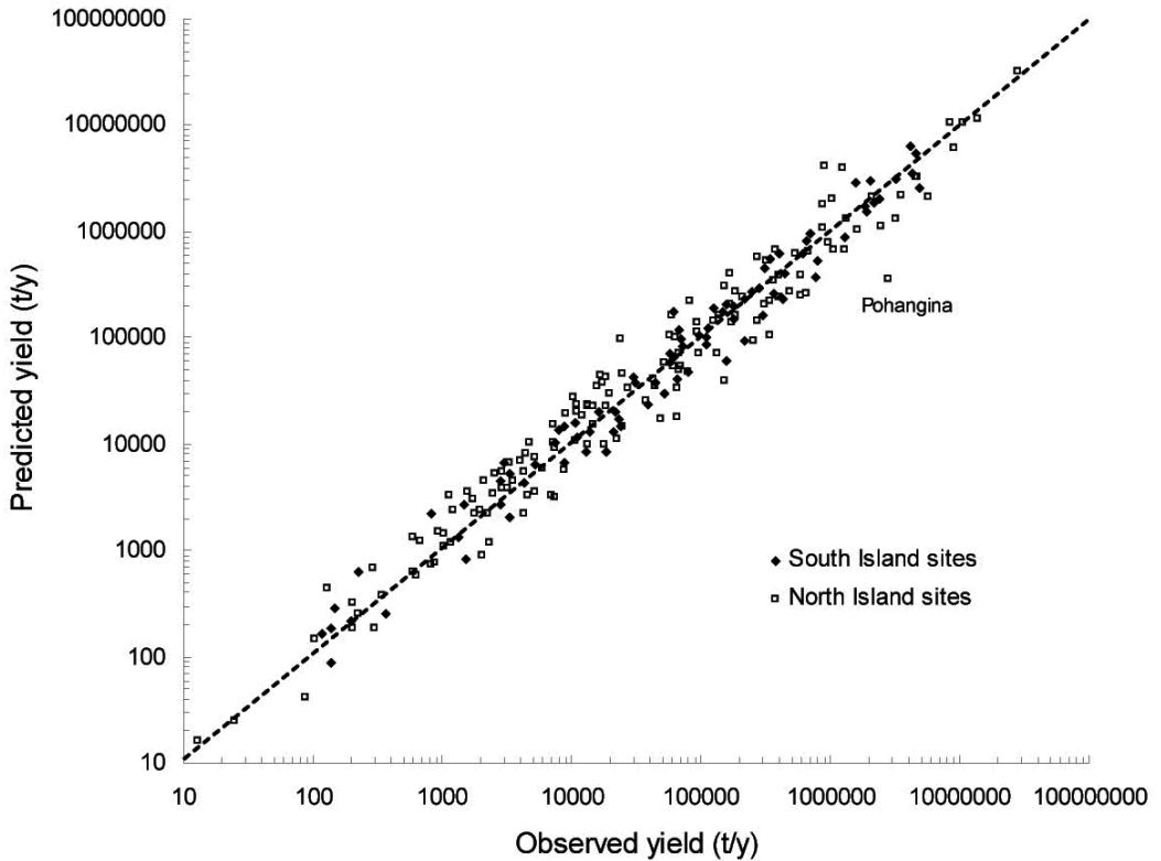
Figure 8 – Final predicted yield versus observed yield, after regional adjustment step.
