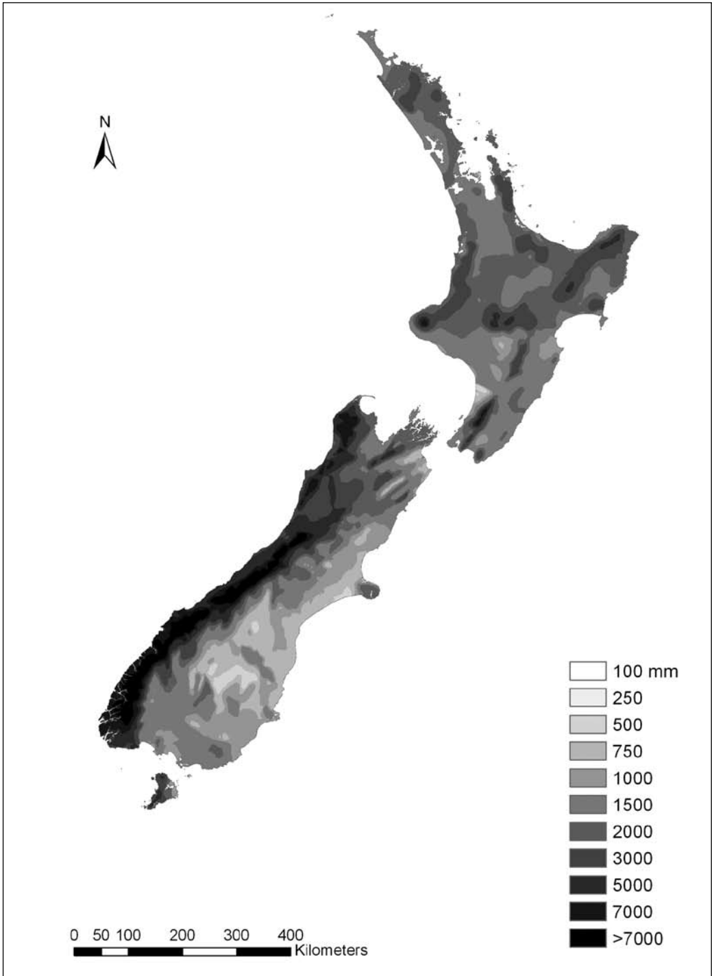
Figure 3 – Raster map of mean annual precipitation (mm) based on 30-year (1961-90) rainfall normal map of Tomlinson and Sansom (1994).
