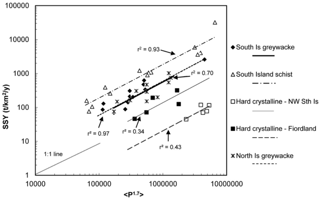
Figure 5 – Relationships between specific suspended sediment yield ( SSY ) and spatially-averaged precipitation to the power of 1.7 ( \langle P^{1.7} \rangle ) for catchment groups with reasonably uniform erosion terrain.
