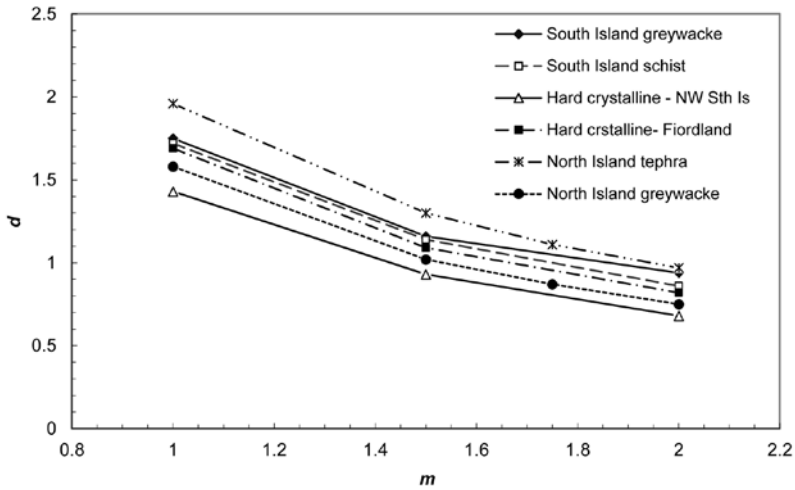
Figure 4 – Exponent d for power-law relations between sediment yield ( SY ) and \langle P^m \rangle A for a range of m for catchment groups with reasonably uniform erosion terrain. \langle P^m \rangle is spatially-averaged m th moment of precipitation; A is catchment area. Power-law relations are linear when d = 1 .
