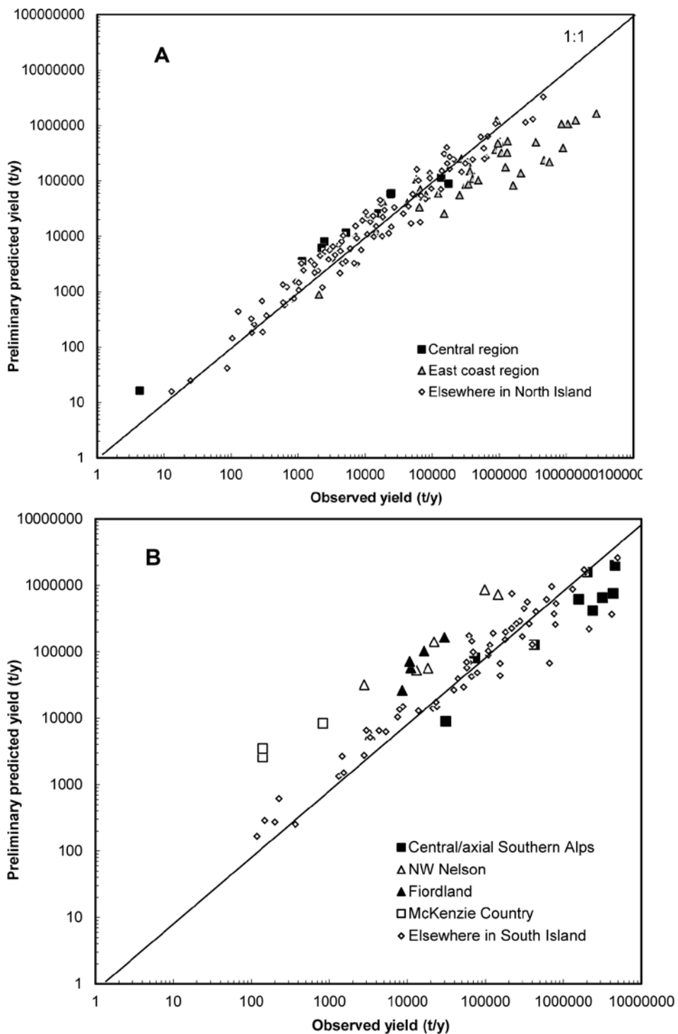
Figure 6 – Preliminary predicted yield versus observed yield, highlighting data for outlier regions. A: North Island, B: South Island.
