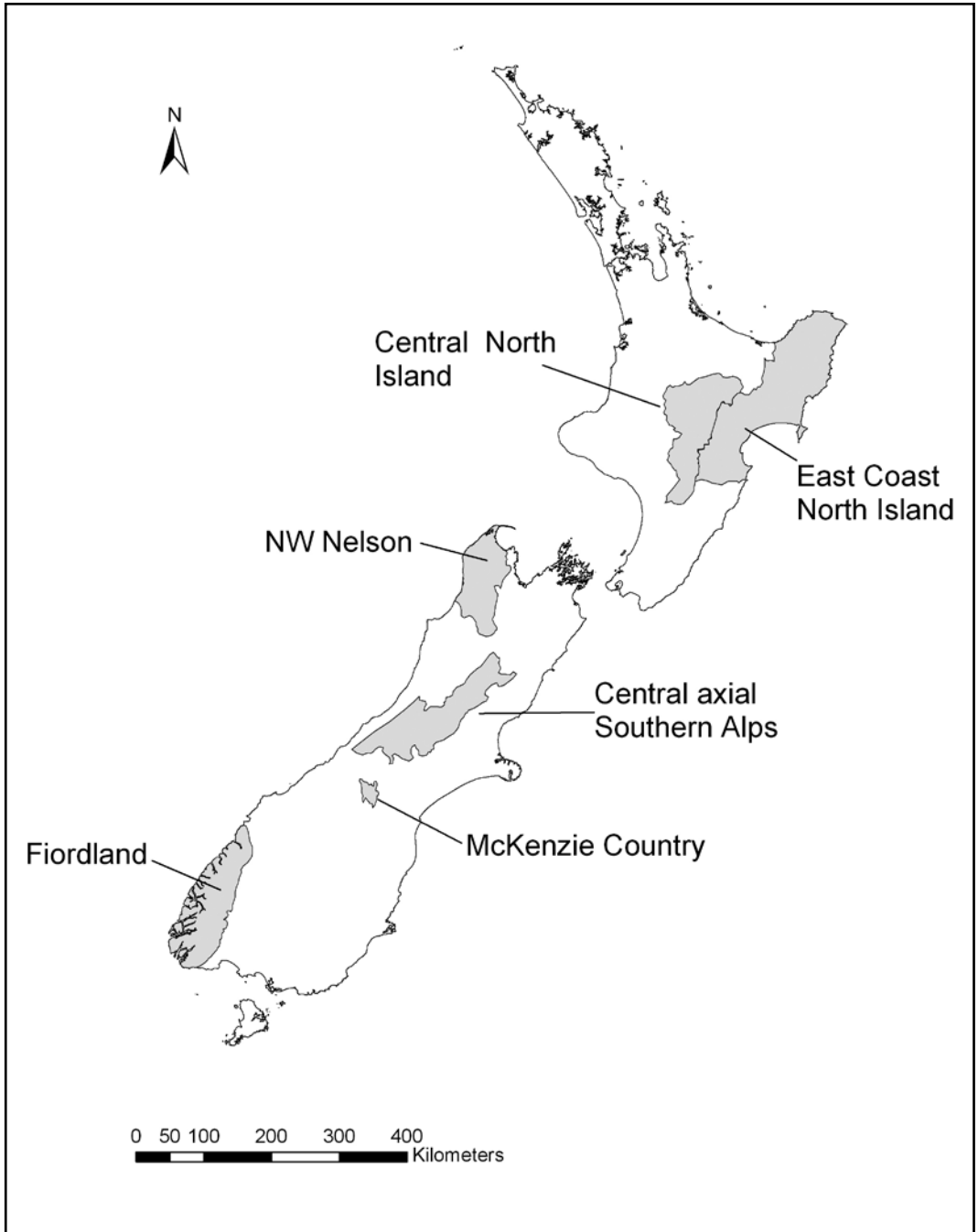
Figure 7 – The six special regions in which the general SSY model required regional adjustment.
