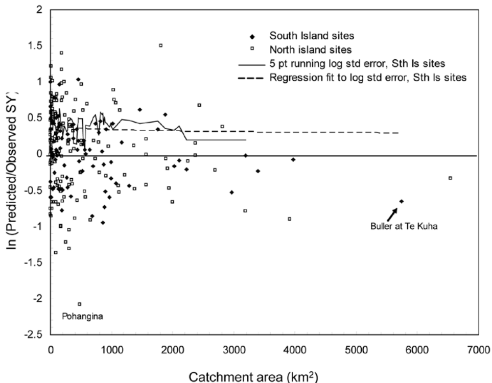
Figure 9 – Final predicted/observed yield versus catchment area.
