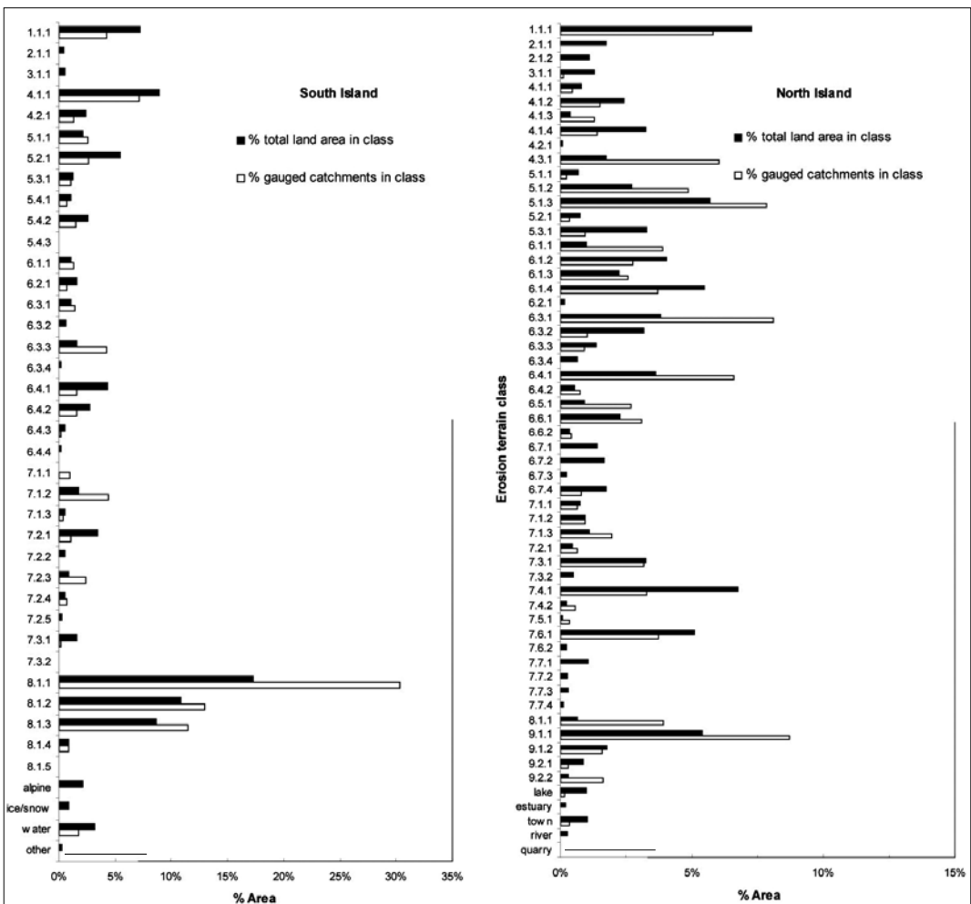
Figure 2 – Percentages of total land area and area of gauged catchments in individual erosion terrain classes for South Island (left) and North Island (right).
