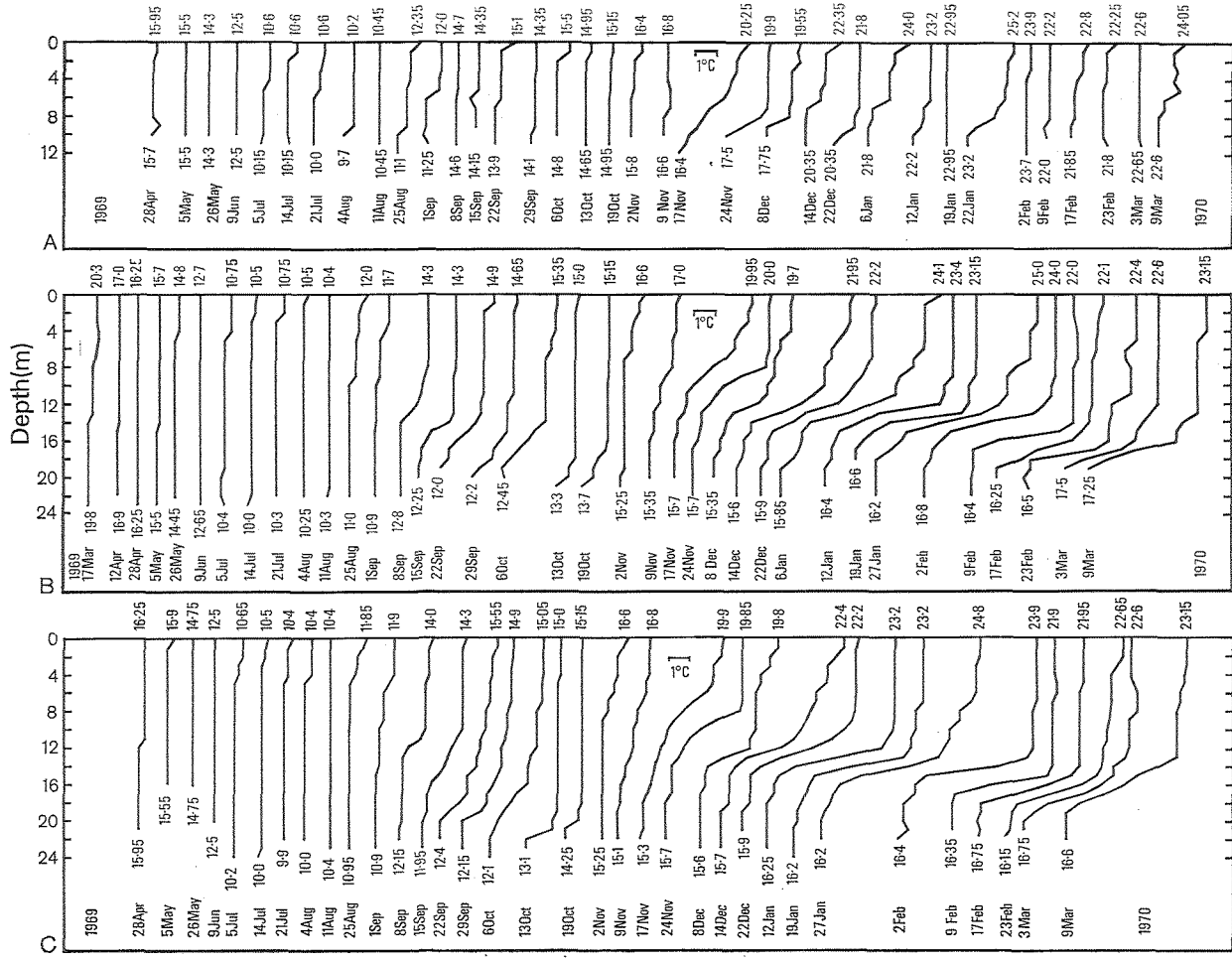
3—Distribution of temperature with depth at the three sampling stations in Lake Ootoa; the surface and bottom temperatures are shown for each trace.
