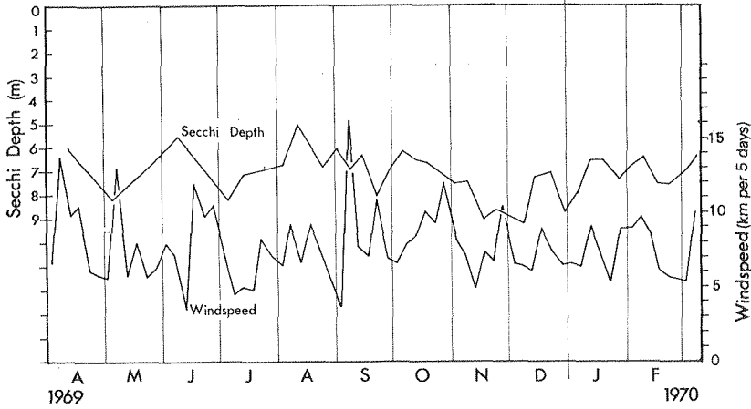
FIG. 6—Seasonal changes in Secchi depth in Lake Ototoa, and windspeed at the neighbouring Woodhill Forest meteorological station. Windspeed is expressed as the number of kilometres run in a 5-day period. Secchi depth is significantly correlated with windspeed in the previous 5-day period ( r = -0.406 , P < 0.02 , n = 35 ).
