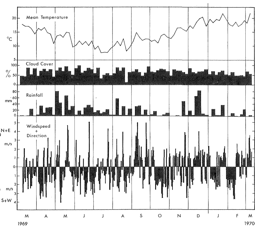
Fig. 2.—Weather March 1969–March 1970 at the Woodhill Forest meteorological station, to the south of Lake Ototoa.
