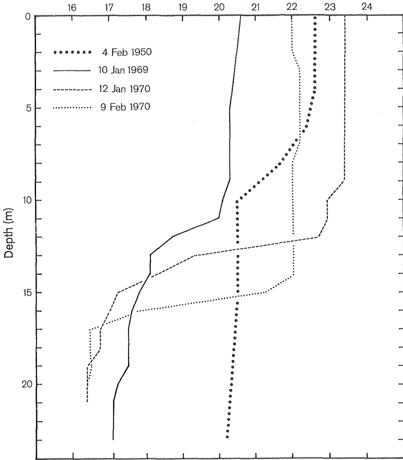
FIG. 4—Thermocline depth in Lake Ototoa during the summers of different years: 1950 from Cunningham et al. (1953); 1969 from a preliminary visit by the author; 1970 from the present study.
