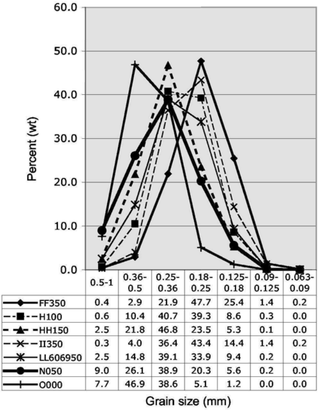
Fig. 6 Grain-size distribution for the seven laboratory-analysed sand-flat sands. Important features are the considerable quantities of sand coarser than 0.36 mm (i.e., not derived from Farewell Spit), and the wide variation between samples. The table below the graph shows weight percentages for each sand in the different size categories along the rows, while comparison up and down columns illustrates the wide variability in weight percent in each size category.
