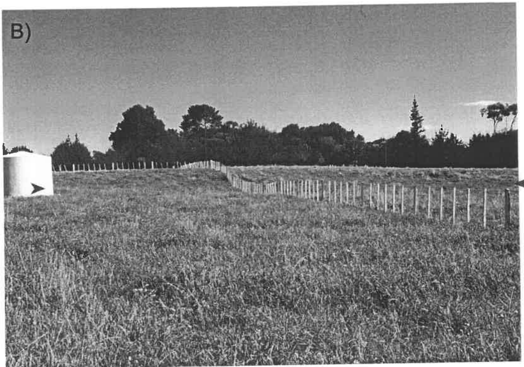
Fig. 5. Photographs looking northwest across the 1-2 m high, southeast-facing, scarp of the Northern Ohariu fault, Old Hautere Road area. Bold arrows show fault's location. Displaced alluvial terrace in photographs is Ohakean in age (about 10 000-15 000 years old). A) Photo taken about 300 m west-southwest of Old Hautere Road (grid ref. S25 909 437). Area shown in this photo is encompassed by that in Fig. 4. B) Photo taken about 200 m northeast of Otaki Gorge Road, between Otaki Gorge Road and the Otaki River (grid ref. S25 925 446). Photo: R. Van Dissen, Institute of Geological & Nuclear Sciences.
