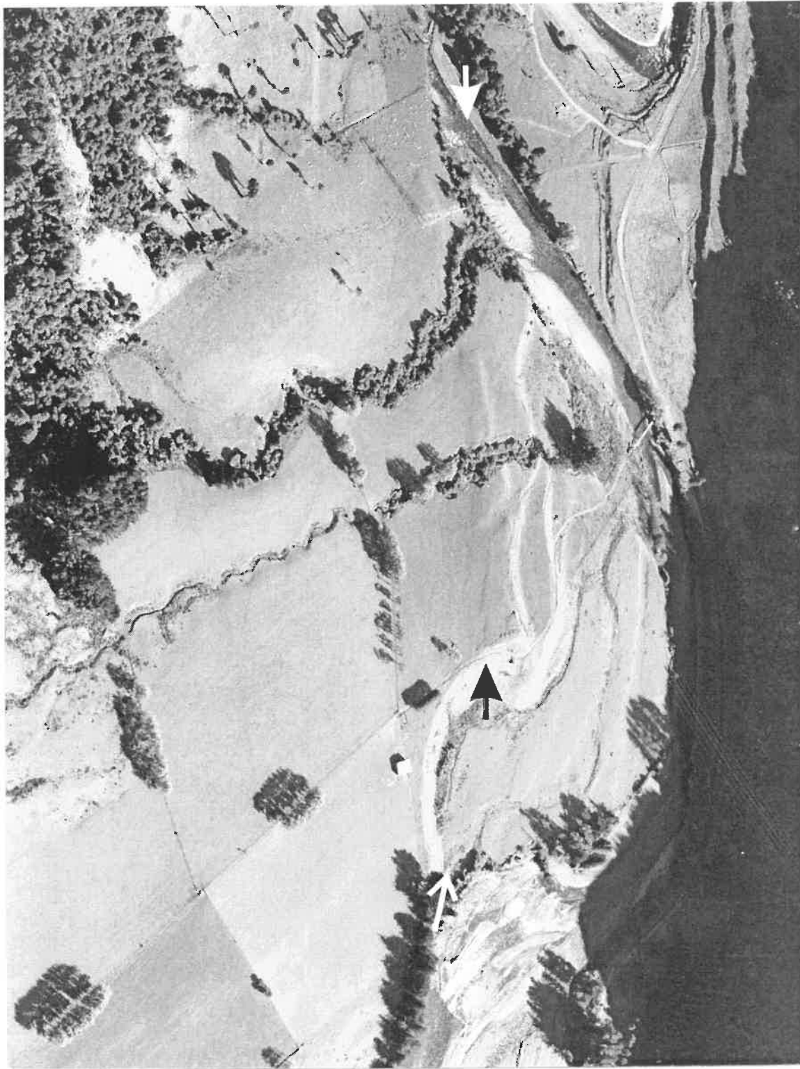
Fig. 12. Aerial photograph looking northwest across the scarp of the Northern Ohariu fault, Poads Road, Ohau River area (grid ref. S25 081 579). Bold arrows show the fault's location across Ohakean age terrace, and finer arrow shows location of possible scarp on Holocene degradational terrace. The photograph shown in Fig. 11 was taken just to the left (southwest) of this photo.
