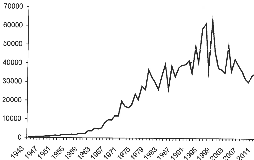
Fig. 1. Total numbers of South Island Oystercatchers counted in winter at Manukau Harbour and the Firth of Thames, 1943–2011.
