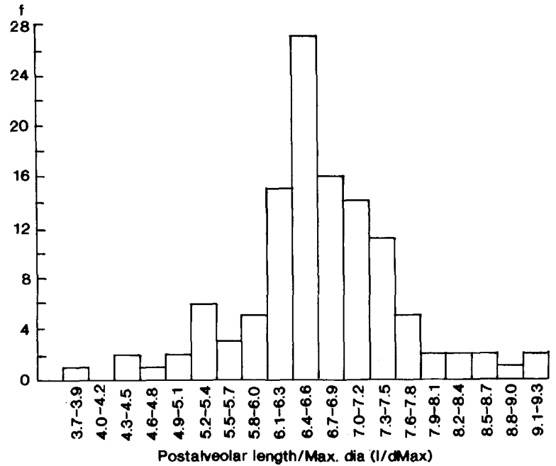
Fig. 51 Frequency distribution of indices of guard robustness ( l/dMax ) in pre-adult Belemnopsis aucklandica . n = 117, \bar{x} = 6.7, \sigma_{n-1} = 9.1.
