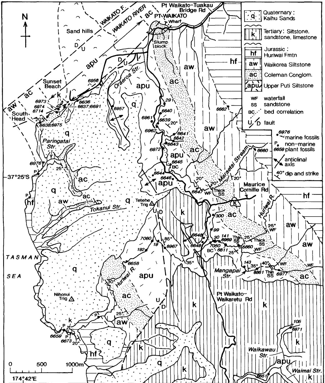
Fig. 3 Geology and fossil localities south and west of Port Waikato. Base map from Purser (1961, map 3). Map based on Purser (1961), Waterhouse (1978), unpublished maps by R. M. Briggs, C. S. Nelson and J. Gillespie (University of Waikato), and additional fieldwork by A.B.C. All localities containing belemnites and ammonites are shown; many also contain Buchia spp.
