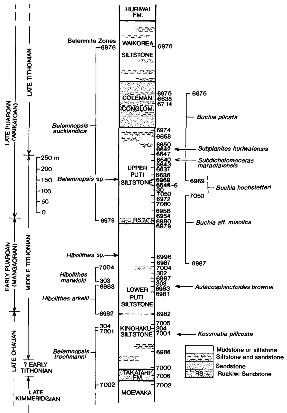
Fig. 10 Composite stratigraphic column for Late Ohauan (part) and Early and Late Puarooan (Mangaoran and Waikatoan) Substages, based on outcrop near Okahu and Moewaka Streams (Fig. 2) and south and west of Port Waikato (Fig. 3). International correlations are from Stevens (1997). RS = Ruakiwi Sandstone. Fossil localities are in approximate relative stratigraphic positions. Known stratigraphic ranges of belemnites and bivalves, and stratigraphic position of ammonite occurrences, are indicated.
