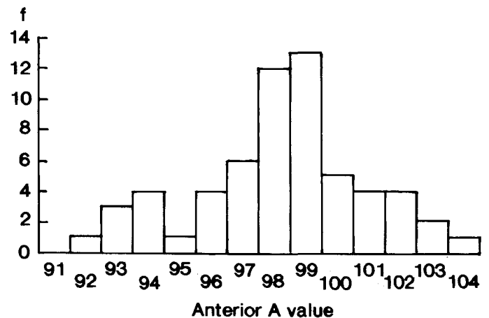
Fig. 16 Frequency distribution of indices of anterior flattening (AA) in adult Belemnopsis aucklandica . n = 60 , \bar{x} = 98.2 , \sigma_{n-1} = 2.7 .
