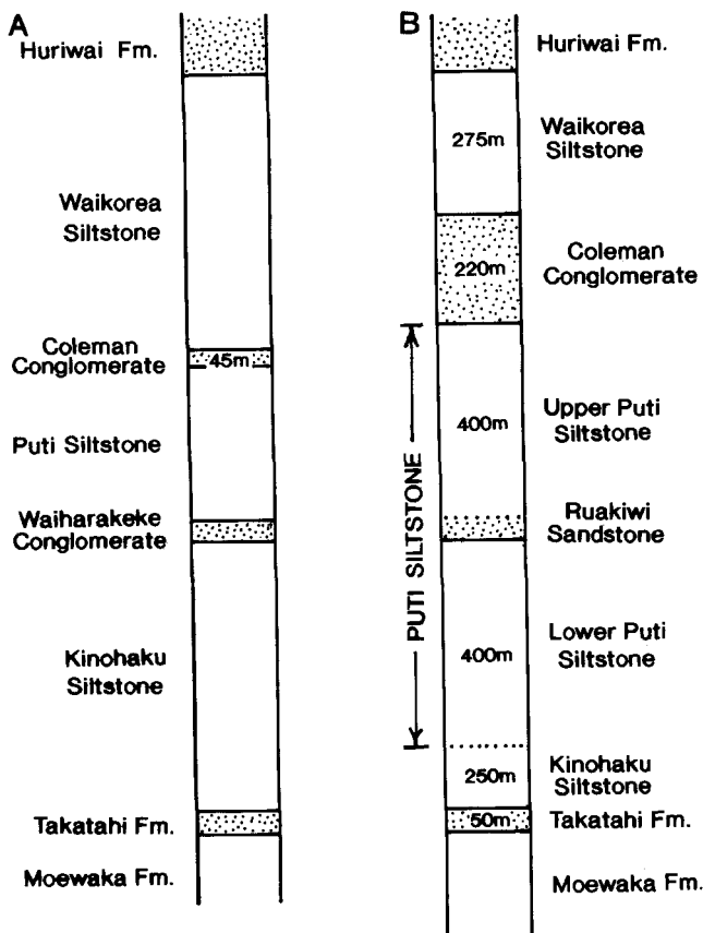
Fig. 11 Alternative correlations of the Late Ohauan–Puarooan sequence at Port Waikato: A , from Waterhouse (1978). B , correlations proposed in this paper. The provisional boundary between the Kinohaku Siltstone and overlying formation does not indicate a lithological change. It is based on paleontology and probably correlates with a horizon near the top of the Kinohaku Siltstone at Kawhia Harbour. The Waiharakeke Conglomerate occurs at and above this point at Kawhia but is not indicated by coarse sediments at Port Waikato.
