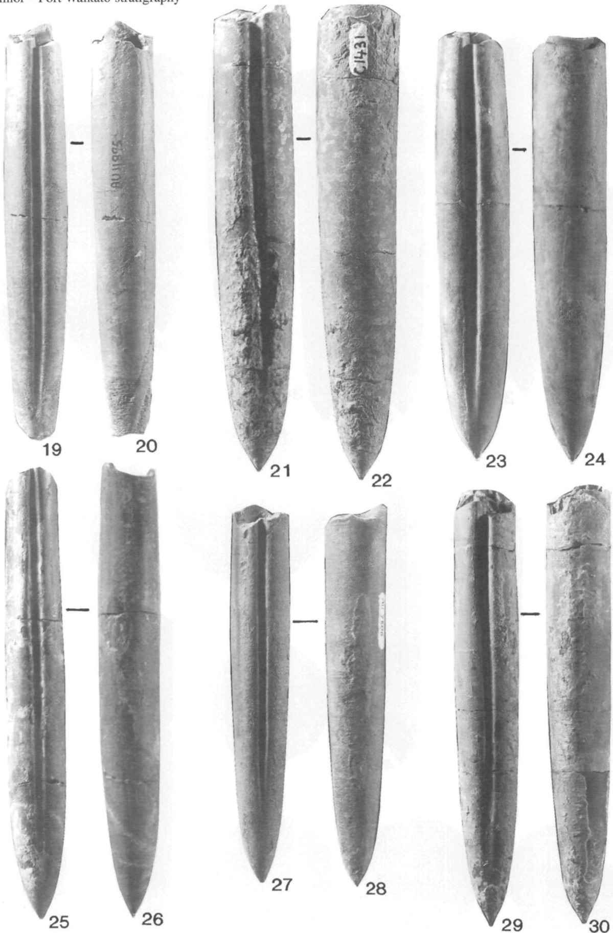
Fig. 19–30 Adult Belemnopsis aucklandica (Hochstetter). All specimens are from Upper Puti Siltstone. 19, 20 (C1867), R13/f99. 21, 22 (C1431), R13/f6961. 23, 24 (C1868), R13/f7080. 25, 26 (C1869), R13/f6973. 27, 28 (C1870), R13/f6636. 29, 30 (C1373), R13/f6961. C1867 (Fig. 19, 20) resembles the holotype in morphology and preservation, although it is slightly larger. C1431, C1868, C1373 (Fig. 21–24, 29, 30), are particularly large specimens. C1869 (Fig. 25, 26) originally figured as Belemnopsis aff. aucklandica by Challinor (1970).
