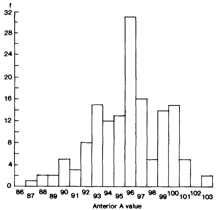
Fig. 53 Frequency distribution of indices of anterior flattening (AA) in pre-adult Belemnopsis aucklandica . n = 149, \bar{x} = 95.8, \sigma_{n-1} = 3.2.
