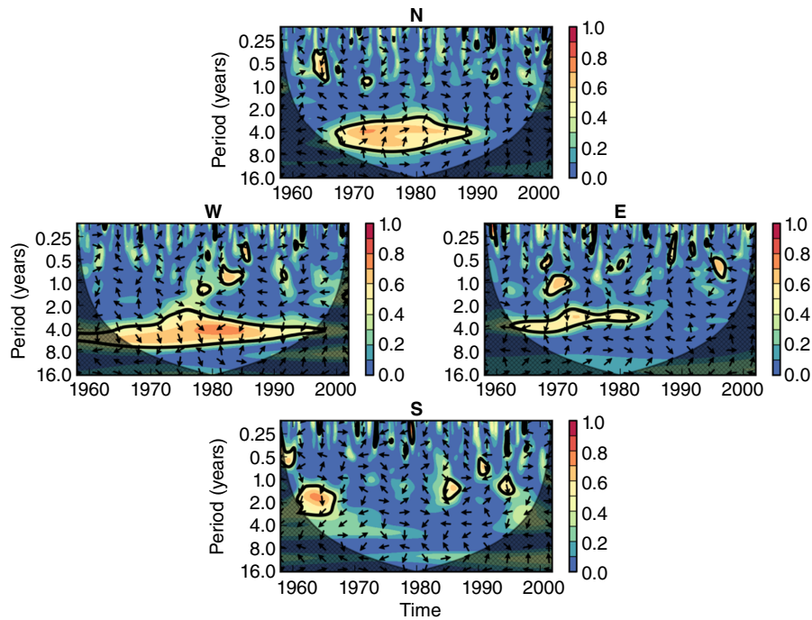
Figure 12. Squared wavelet coherence spectra of monthly anomalies of storm cluster indices with monthly anomalies of the SOI. Thick contours represent 90% confidence levels, while hatched areas represent the cone-of-influence. In phase and antiphase signals are represented by arrows pointing upwards and downwards, respectively. Arrows pointing rightwards represent the ENSO preceding SWCs, whereas the converse is true for arrows pointing leftwards. The letters N, W, E, and S on top of each plot stand for north, west, east, and south coasts, respectively. [Colour figure can be viewed at wileyonlinelibrary.com ].
