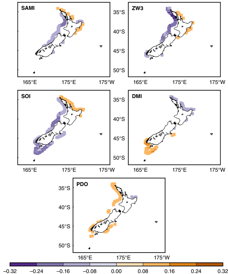
Figure 7. Correlations of monthly anomalies between storm cluster indices and climate indices. Correlations were carried out at the model grid points on the 200 m isobath over the period 1958–2001 for the SAMI, SOI, DMI, and PDO Index, and over the period 1979–2001 for the ZW3 Index. Only statistically significant values at the 95% confidence level are displayed. [Colour figure can be viewed at wileyonlinelibrary.com ].
