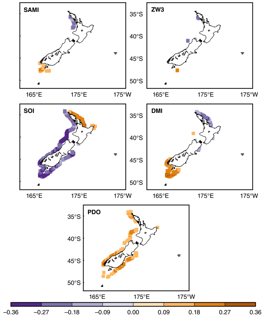
Figure 8. Correlations of seasonally averaged monthly anomalies between storm cluster indices and climate indices lagged by one season. Correlations were carried out at the model grid points on the 200 m isobath over the period 1958–2001 for the SAMI, SOI, DMI, and PDO Index, and over the period 1979–2001 for the ZW3 Index. Only statistically significant values at the 95% confidence level are displayed. [Colour figure can be viewed at wileyonlinelibrary.com ].
