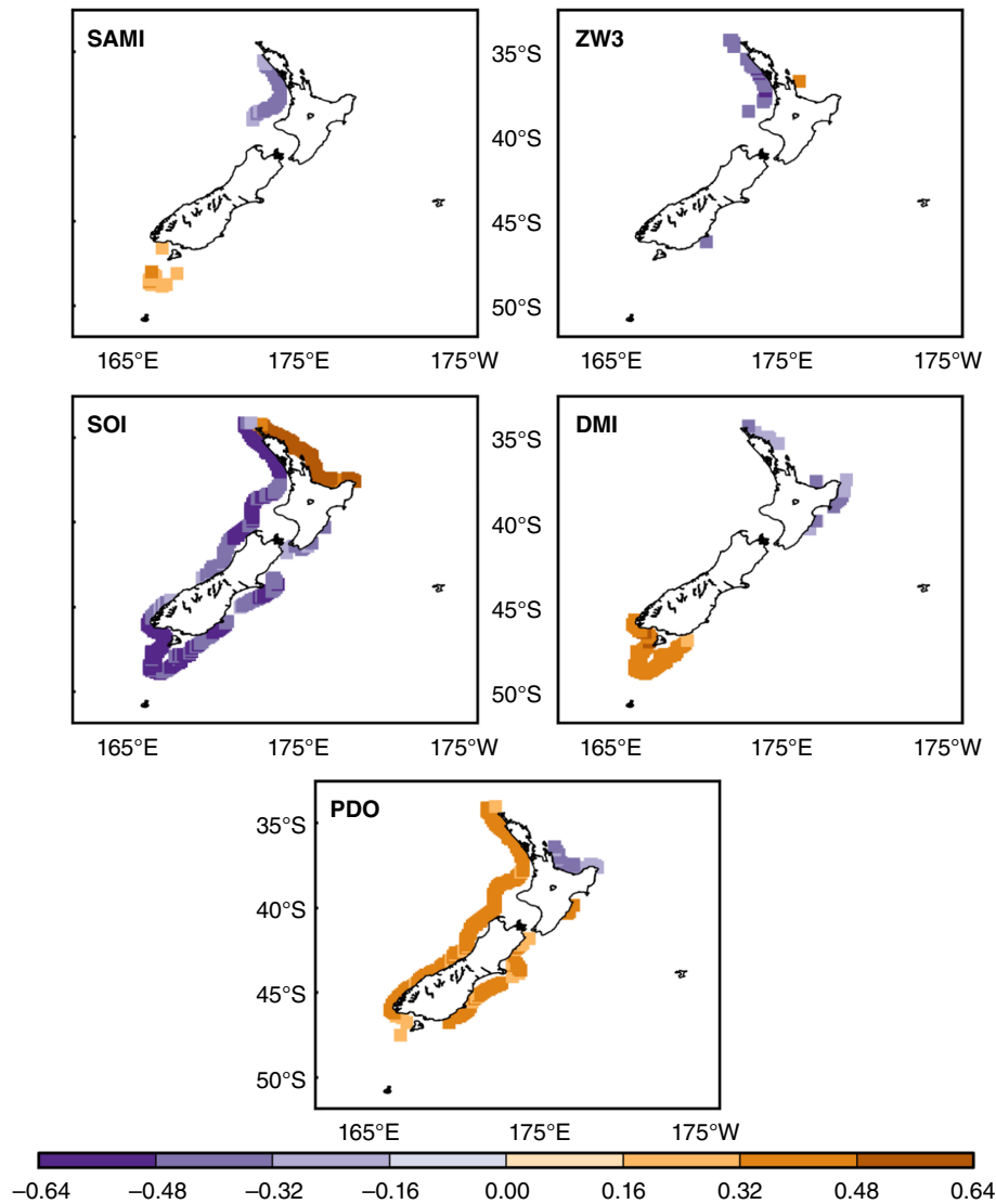
Figure 9. Correlations of annually averaged monthly anomalies between CSE per cluster and climate indices. Correlations were carried out at the model grid points on the 200 m isobath over the period 1958–2001 for the SAMI, SOI, DMI, and PDO Index, and over the period 1979–2001 for the ZW3 Index. Only statistically significant values at the 95% confidence level are displayed. [Colour figure can be viewed at wileyonlinelibrary.com ].
