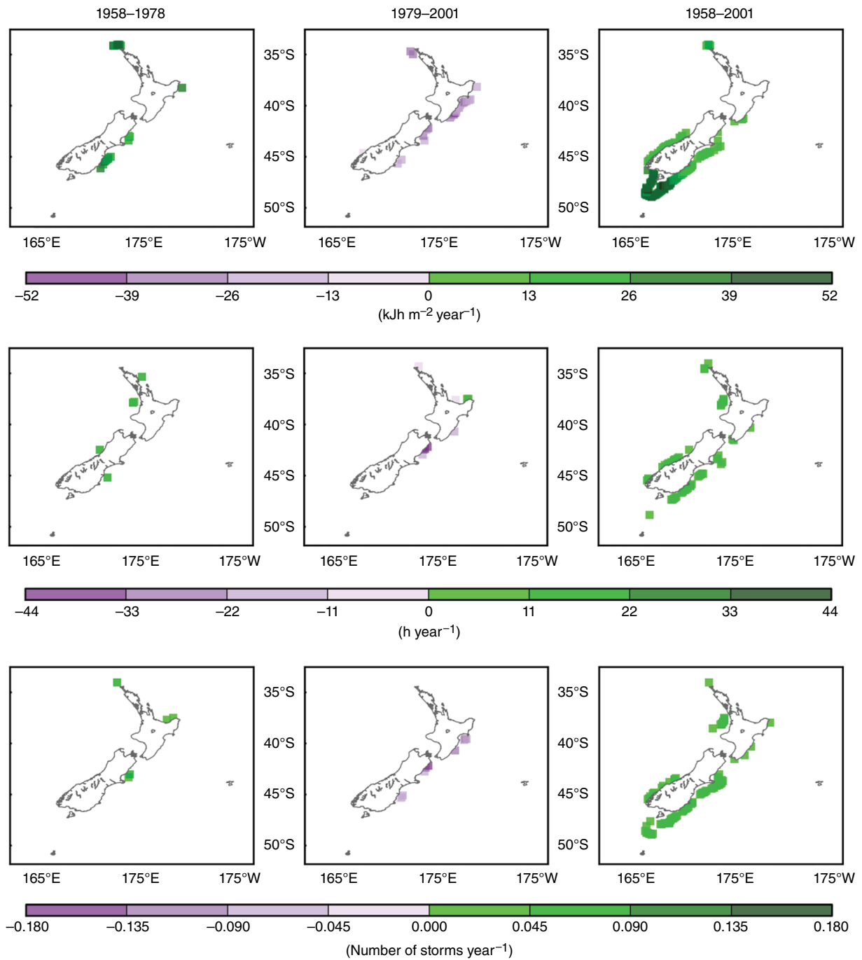
Figure 5. Monotonic trends in SWC parameters, calculated for the pre-satellite period (1958–1978, left column), satellite period (1979–2001, middle column), and long-term period (1958–2001, right column). Top row: CSE (in kilo Jh m -2 ); middle row: cluster duration; bottom row: number of storms within the cluster. Trends were calculated from annual averages of the cluster parameters using the Mann–Kendall test and the Theil–Sen estimator. Only statistically significant values at the 95% confidence level (calculated using p -value) are displayed. [Colour figure can be viewed at wileyonlinelibrary.com ].
