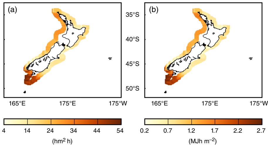
Figure 4. Measures of the potential for cluster-induced coastal erosion: (a) average SPI per cluster (in \text{hm}^2 \text{h} ); (b) average CSE per cluster (in \text{MJh m}^{-2} ). The averages were calculated using all SWCs occurred during the period 1958–2001 for each model grid point on the 200 m isobath. [Colour figure can be viewed at wileyonlinelibrary.com ].
