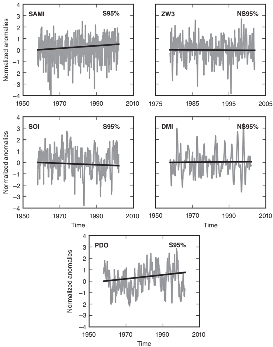
Figure 6. Monotonic trends in normalized anomalies of climate indices: SAMI, ZW3 Index, SOI, DMI, and PDO Index. The anomalies of climate indices were normalized by the standard deviation. Trends were computed for the period 1979–2001 for the ZW3 Index, and for the period 1958–2001 for the other indices. S95% and NS95% stand for statistically significant and non-significant at the 95% confidence level, respectively.
