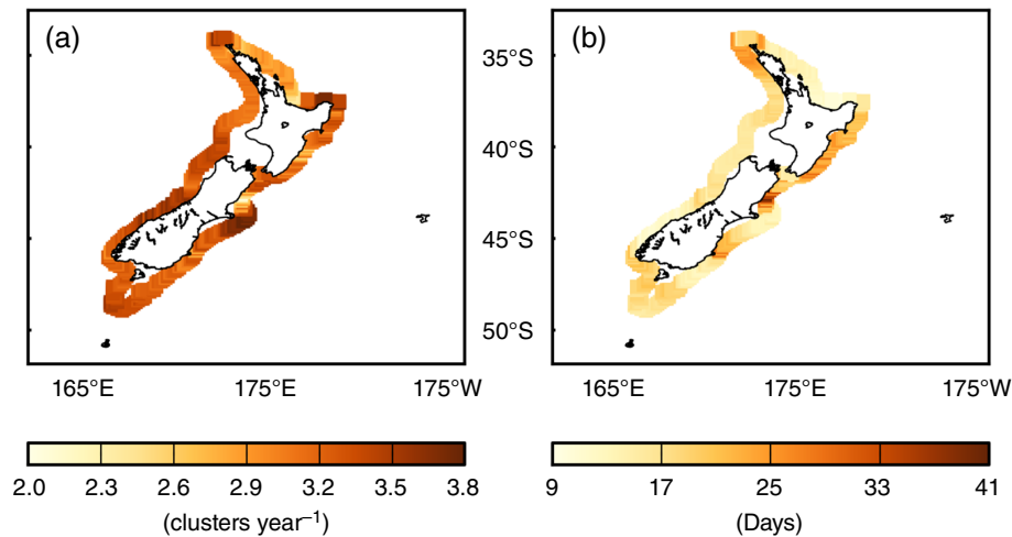
Figure 3. Considering the period 1958–2001: (a) annual average number of SWCs; (b) average SWC duration. The averages were calculated at the model grid points on the 200 m isobath. [Colour figure can be viewed at wileyonlinelibrary.com ].
