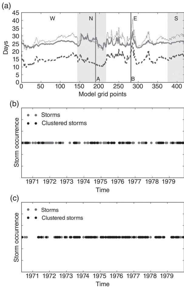
Figure 2. (a) Statistics computed for time series of storm wave occurrence at the 418 model grid points on the 200 m isobath: half of the index of dispersion of time intervals between storm peaks (dashed line), mean interval between storm peaks (solid line), and standard deviation of the time interval between storm peaks (dotted line). Vertical lines A and B mark the largest and smallest differences between the mean interval between storm peaks and half of the index of dispersion; the locations of the model grid points associated with these differences are displayed in Figure 1 as A and B. W, N, E, and S stand for west, north, east, and south, respectively, delimited according to Figure 1. Shaded and non-shaded areas of the graph comprise the model grid points along each section of the coastline (W: 0–143; N: 144–216; E: 217–375; S: 376–417), with 0 being located on the southwestern coast (triangle in Figure 1) and the subsequent numbers follow a clockwise rotation; (b) time series of occurrence of storms and clustered storms at site A; (c) time series of occurrence of storms and clustered storms at site B. Grey circles represent storm waves, whereas black circles indicate storm waves pertaining to clusters.
