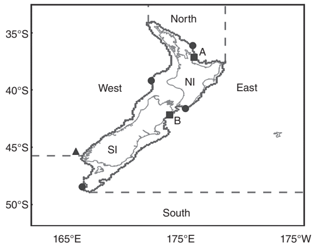
Figure 1. Regional domain of the 45-year (1957–2002) wave hindcast. Filled circles represent the locations used in the wavelet spectral analysis. Filled squares A and B indicate the sites used as examples for showing time series of occurrence of clustered storms in Figures 2(b) and (c), respectively. Grey dots illustrate the model grid points on the 200 m isobath, with the filled triangle marking the first point (0) of the sequence of Figure 2(a). Dashed lines represent coastline delimiters, plotted here as a guide for Figure 2(a). NI and SI stand for North Island and South Island, respectively.
