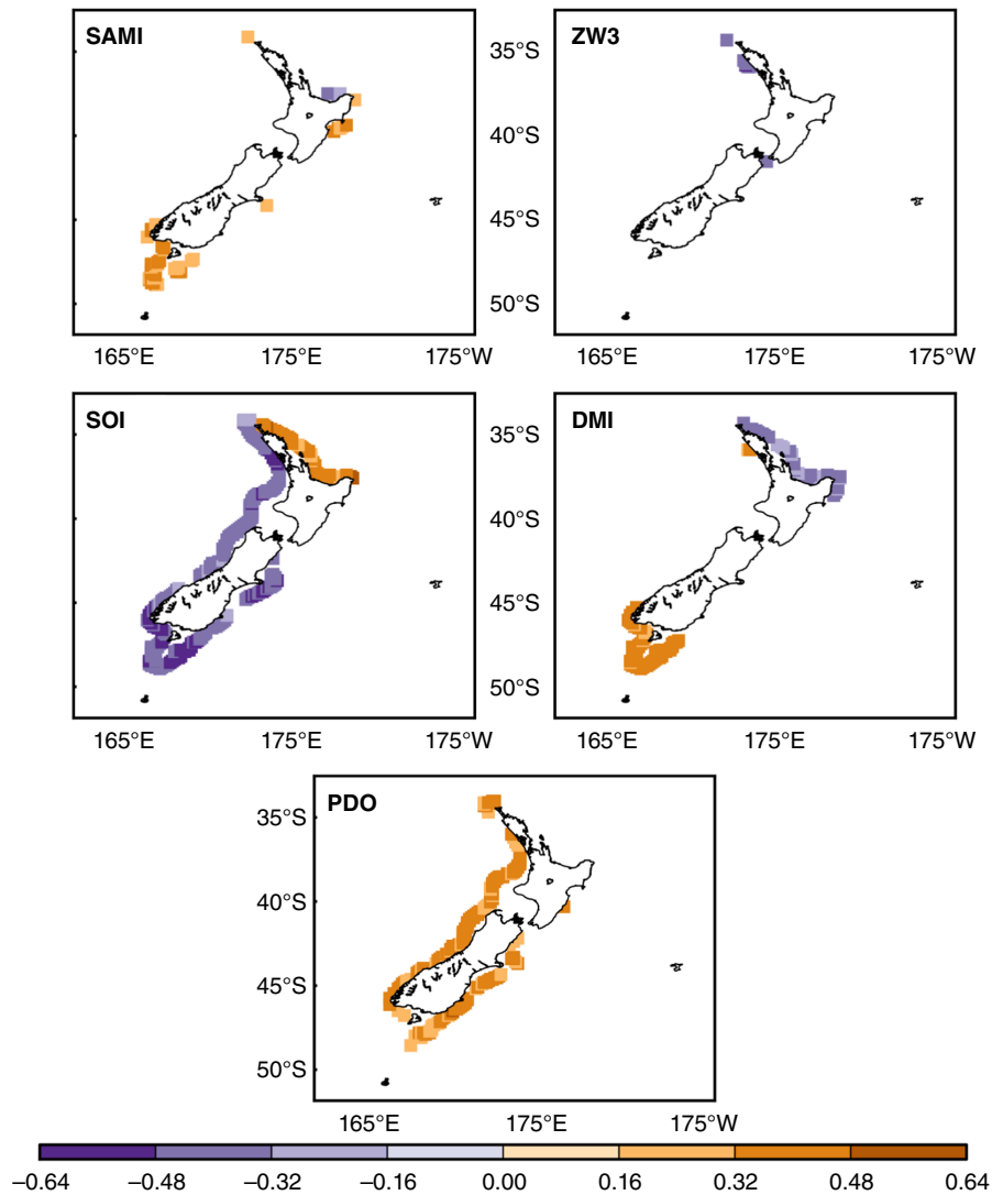
Figure 10. Correlations of annually averaged monthly anomalies between storm cluster duration and climate indices. Correlations were carried out at the model grid points on the 200 m isobath over the period 1958–2001 for the SAMI, SOI, DMI, and PDO Index, and over the period 1979–2001 for the ZW3 Index. Only statistically significant values at the 95% confidence level are displayed. [Colour figure can be viewed at wileyonlinelibrary.com ].
