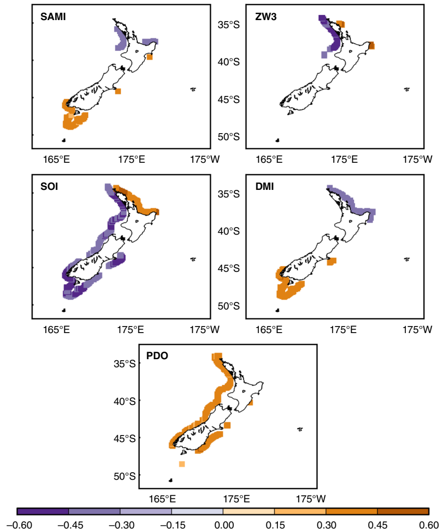
Figure 11. Correlations of annually averaged monthly anomalies between the number of storms within the cluster and climate indices. Correlations were carried out at the model grid points on the 200 m isobath over the period 1958–2001 for the SAMI, SOI, DMI, and PDO Index, and over the period 1979–2001 for the ZW3 Index. Only statistically significant values at the 95% confidence level are displayed. [Colour figure can be viewed at wileyonlinelibrary.com ].
