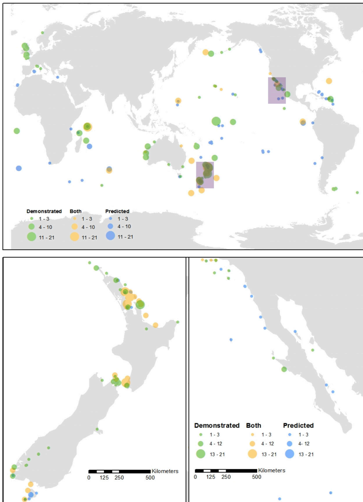
Fig. 1. (Upper) Islands with native fauna populations with demonstrated and/or predicted benefits from invasive mammal eradications. Dot size indicates numbers of populations. New Zealand (Lower Left) and the Gulf of California, Mexico (Lower Right) are featured because they contain some of the highest numbers of eradications and beneficiaries from our collated datasets. Demonstrated beneficiaries include vertebrates and invertebrates; predicted beneficiaries are restricted to critically endangered or endangered birds, mammals, and reptiles on the IUCN Red List.
