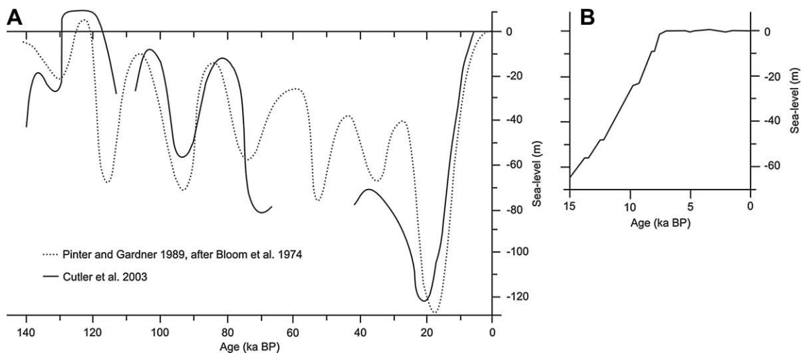
Fig. 3. Sea-level changes in the southwest Pacific region surrounding New Zealand as documented by records from (A) the Huon Peninsula, Papa New Guinea, (B) the New Zealand region (after Carter et al., 2002).
