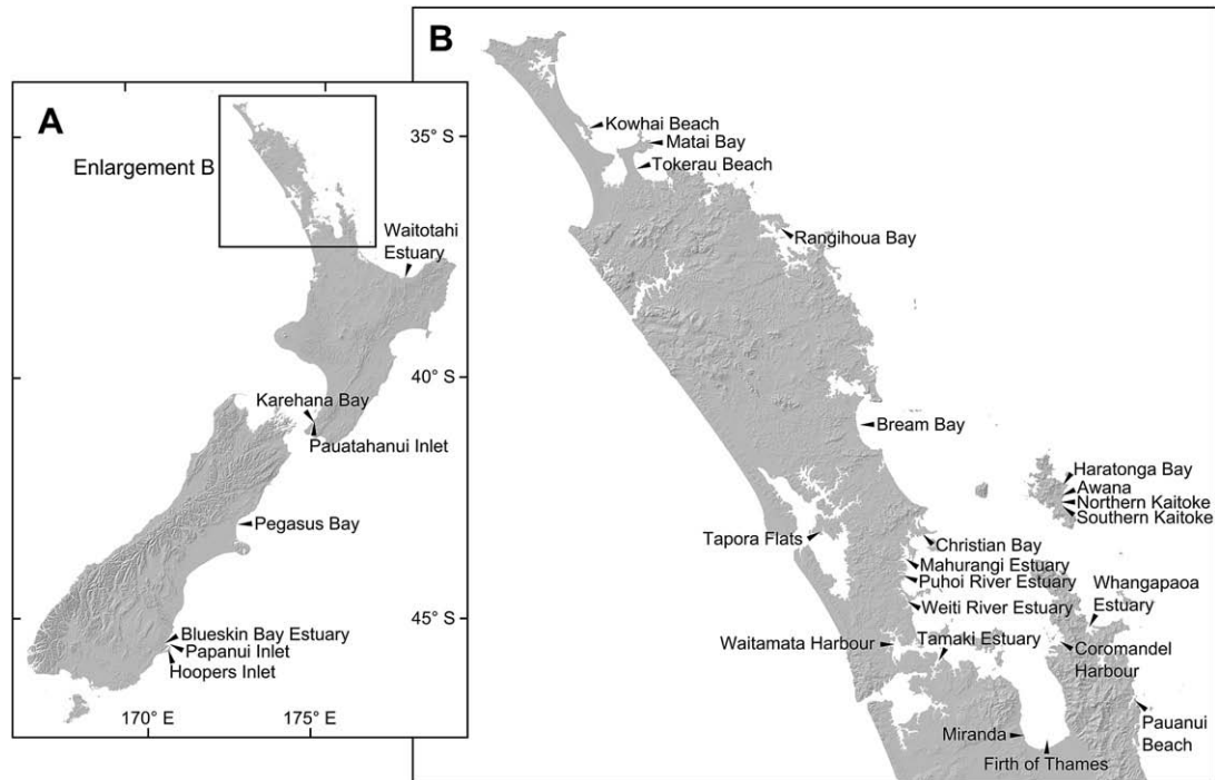
Fig. 4. Map of the spatial distribution of sea-level index points used to compile the revised Holocene sea-level curve for the New Zealand region (Fig. 5).
