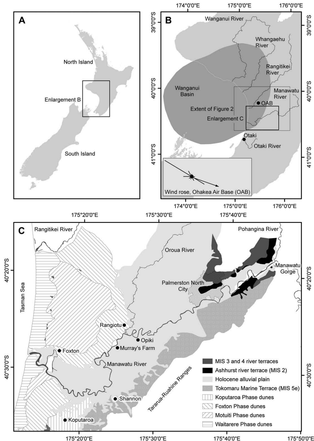
Fig. 1. (A) Contextual map of New Zealand; (B) location map of the Wanganui Basin, regionally significant rivers and localities and location of Fig. 2; (C) quaternary geology of the Manawatu region (after Shepherd, 1987 ).
