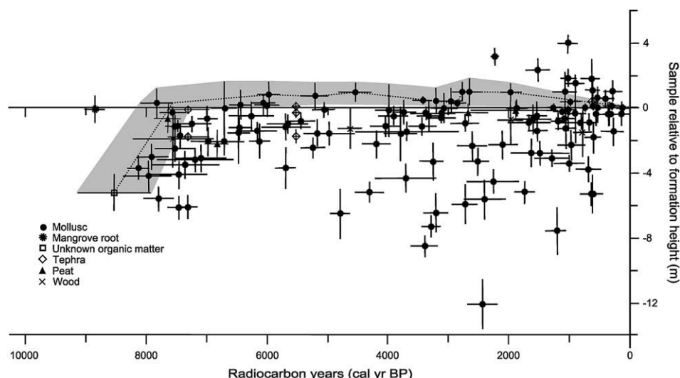
Fig. 5. Revised Holocene sea-level curve for the New Zealand region (after Clement et al., 2008a,b).
