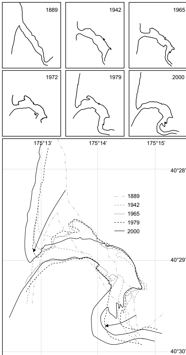
Fig. 6. Time-series map of recent geomorphological change of the modern Manawatu River estuary. 1972 is omitted from the overlay to enhance legibility given the relatively little change in profile from 1965 to 1972.
