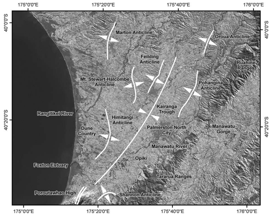
Fig. 2. Fold axes of the Manawatu anticlines overlaid on an Enhanced Thematic Mapper image of the Manawatu region (after Clement and Brook, 2008).
