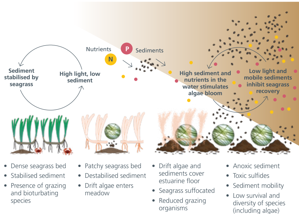
Figure 2.2: Feedback loops in seagrass meadows. Seagrass stabilises sediments in soft-bottomed estuaries and provides vital habitat for estuary ecosystems. Excess sediment blocks light to the seagrass and estuarine floor, and nutrients encourage algae growth. Increased algae, in turn, lowers light levels and prevents seagrass recovery.
