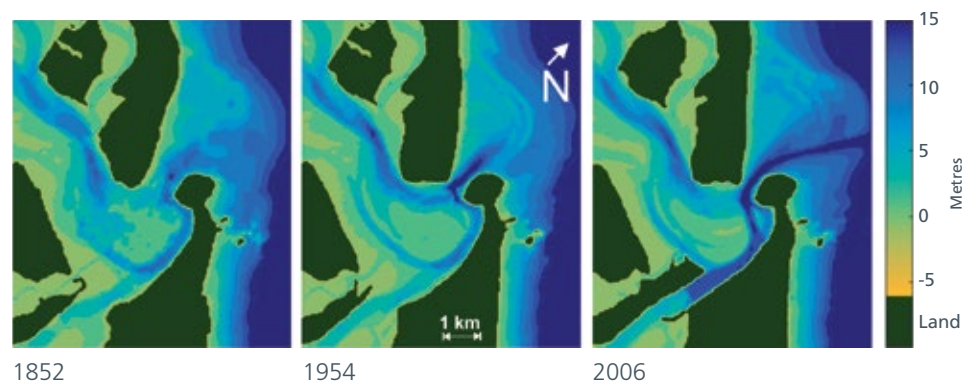
Figure 7.3.3: Tauranga Harbour bathymetric charts showing channel depths prior to construction and reclamation of Sulphur Point (1852), through to 2006.
