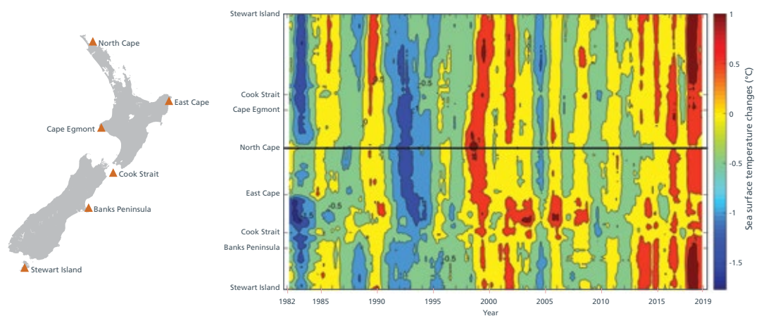
Figure 2.1: Timeseries of annually smoothed temperature changes near New Zealand coasts. A) Reference monitoring stations. B) The y-axis represents the locations monitored running north from Stewart Island along the east coast to North Cape, then south down the west coast. The x-axis represents years from 1982 to 2019. 10
